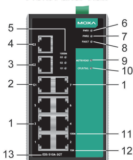
EDS-510A-1GT2SFP Front Panel View
