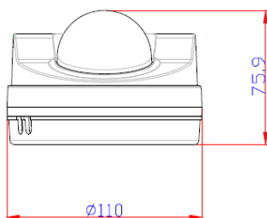
Camera with CO2 adaptor
